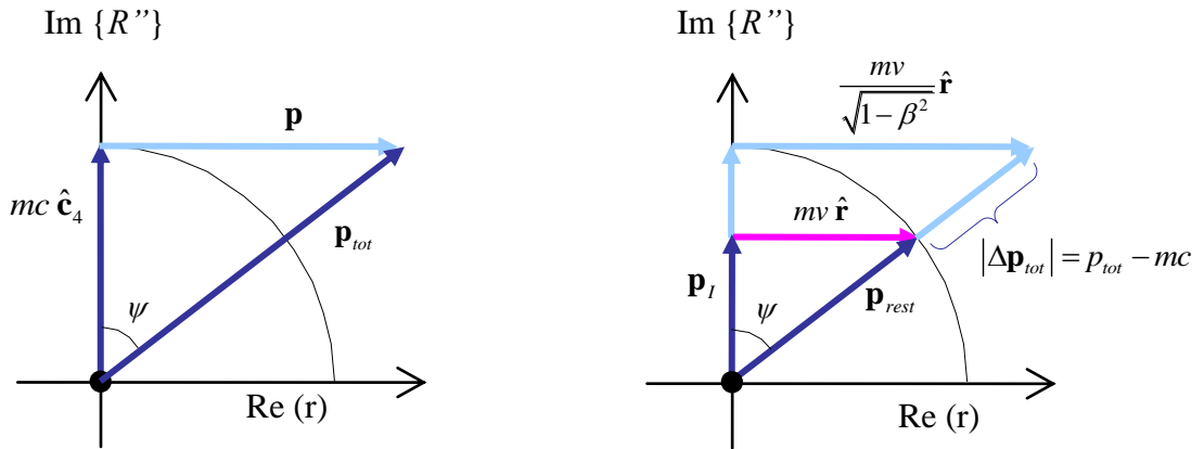
Figure 4. The rest momentum of an object (a) at rest in space and (b) moving at velocity \mathbf{v} in space direction \{r\} .
