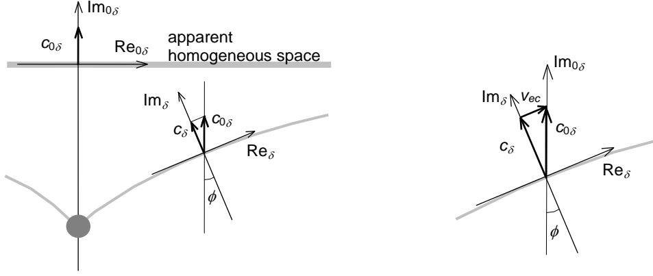
Figure 7. Space is tilted in the fourth dimension close to mass centers in space. Local complex coordinates follow the shape of space, causing the local imaginary axis, Im_{\delta} , to deviate from the direction of the imaginary axis in apparent homogeneous space, Im_{0\delta} . The imaginary velocity of space in the \delta -state, c_{\delta} , is reduced according to the formula c_{\delta} = c_{0\delta} \cos \phi , where \phi is the tilting angle of space in the \delta -state. The orthogonal sum of the local imaginary velocity and the escape velocity, v_{ec} , to apparent homogeneous space is equal to the imaginary velocity of the apparent homogeneous space as illustrated in the picture on the right.
